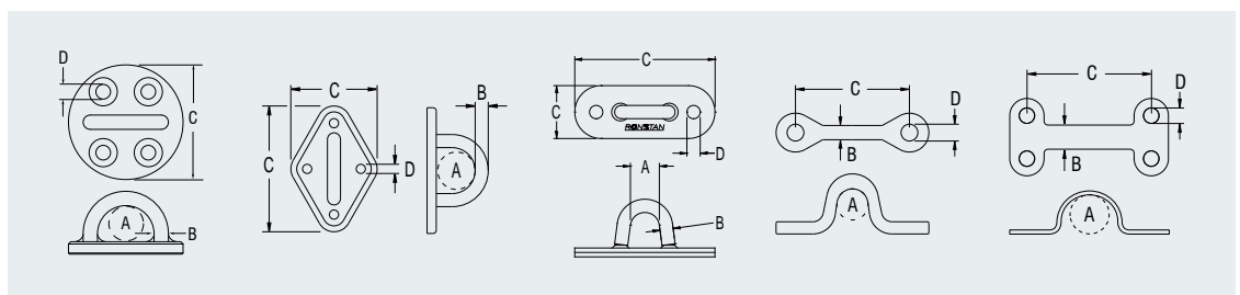
SADDLES - NARROW
